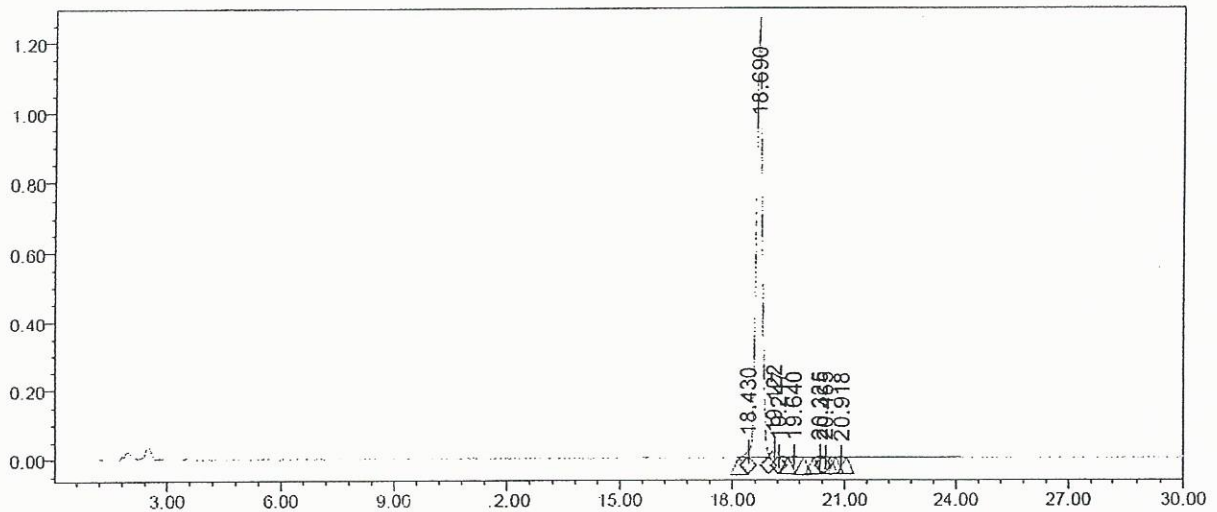
Auto-Scaled Chromatogram
